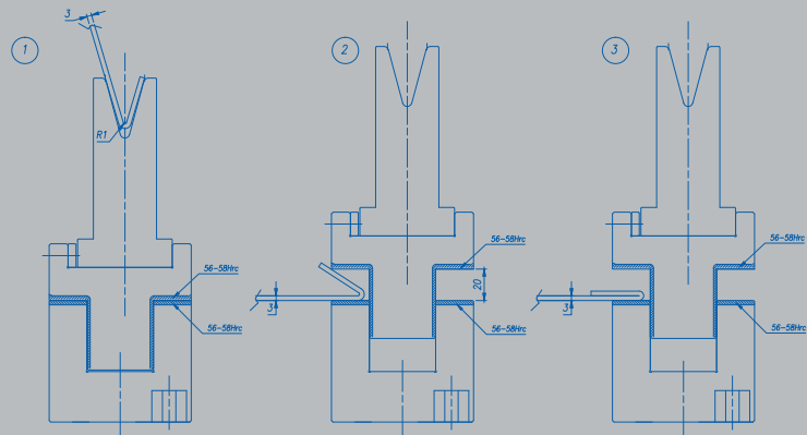
Special hemming table, pneumatically driven
