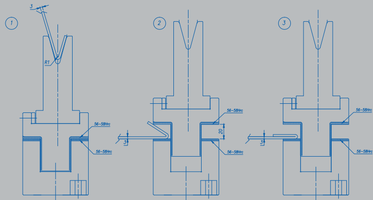
Special hemming table, pneumatically driven
